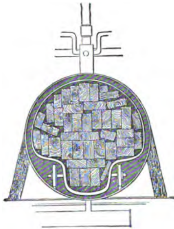
Fig. 310.—Front of an injecting cylinder with a truck laden with wood.
